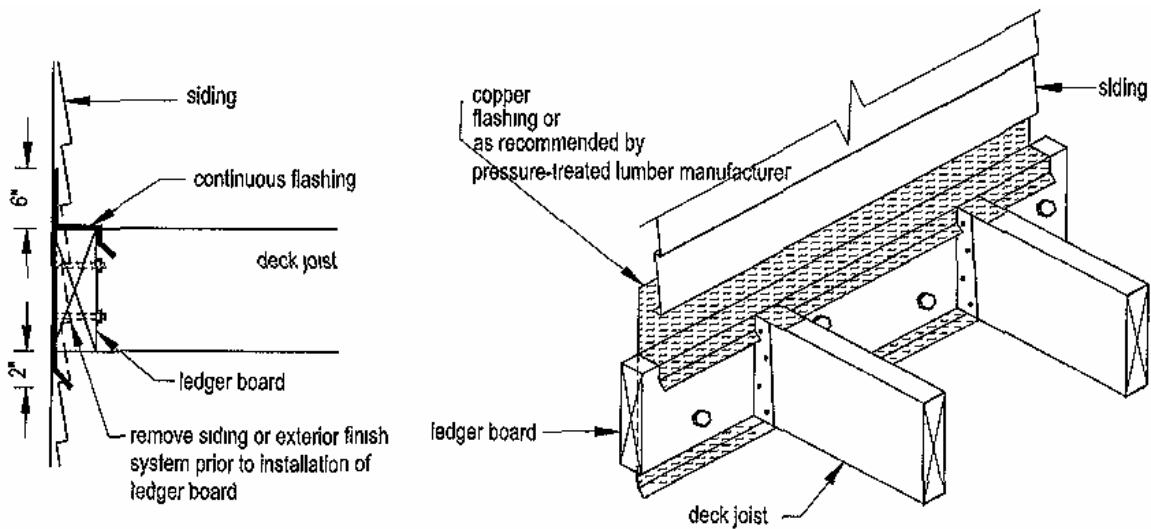
Figure 14: Flashing requirements
