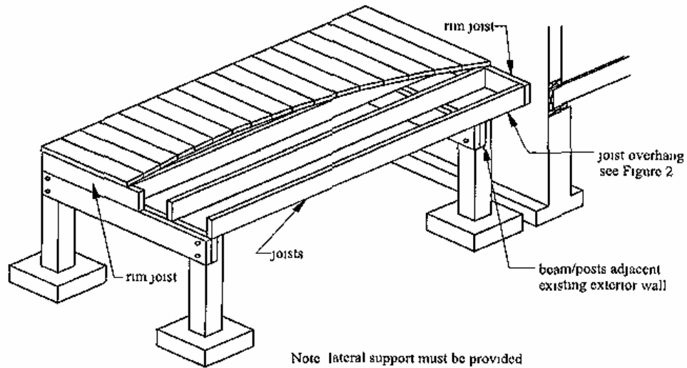
Figure 6: Freestanding deck
