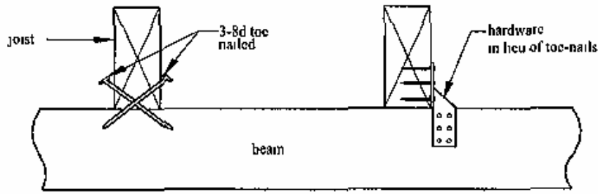
Figure 16: Joist to beam detail
