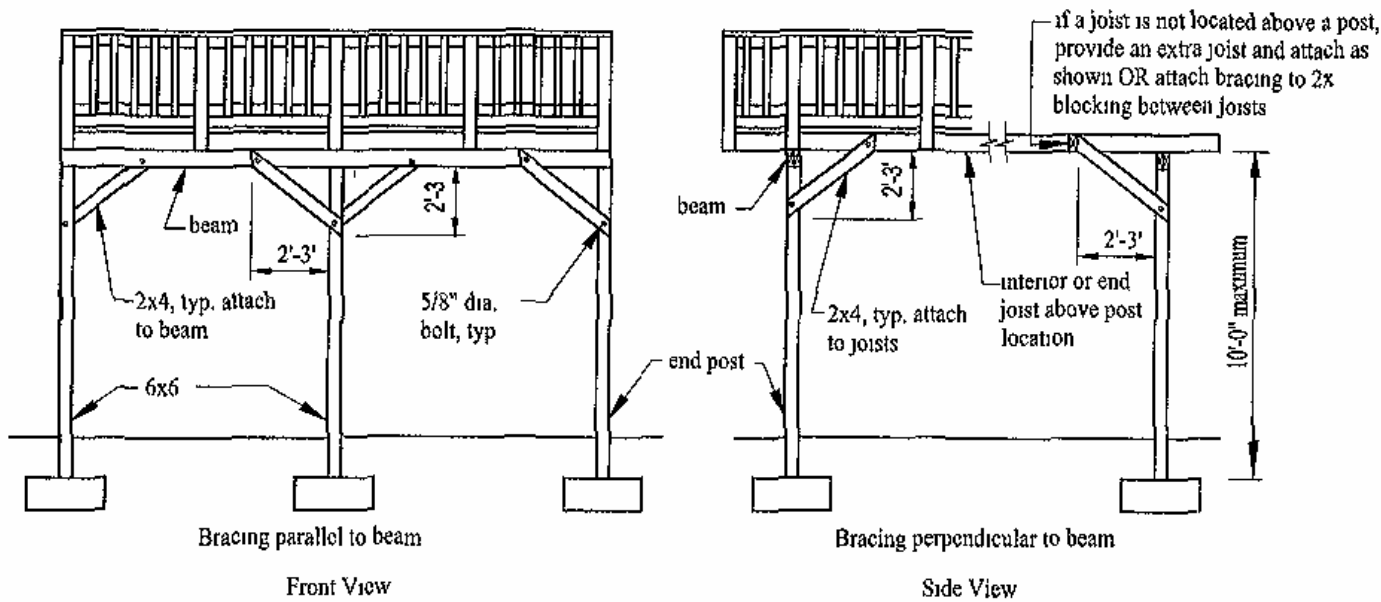
Note: Filler blocks may be required at the beams and joists Figure 15: Bracing for freestanding decks
