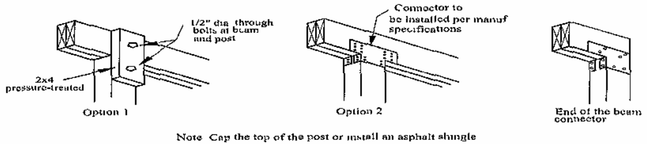
Figure 20: 4x4 inches post-to-beam connection
