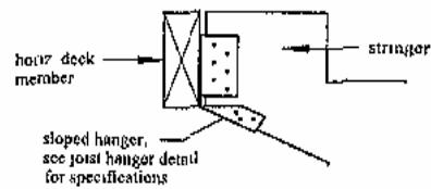
Alternate attachment
