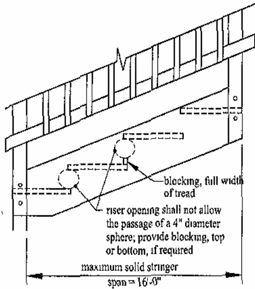
Figure 27: Solid stair stringer detail
