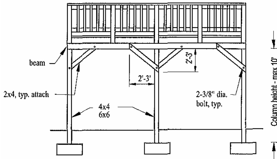
Figure 4: Deck posts
