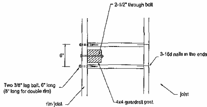
Figure 25: Plan (top) view-Interior guardrail post
