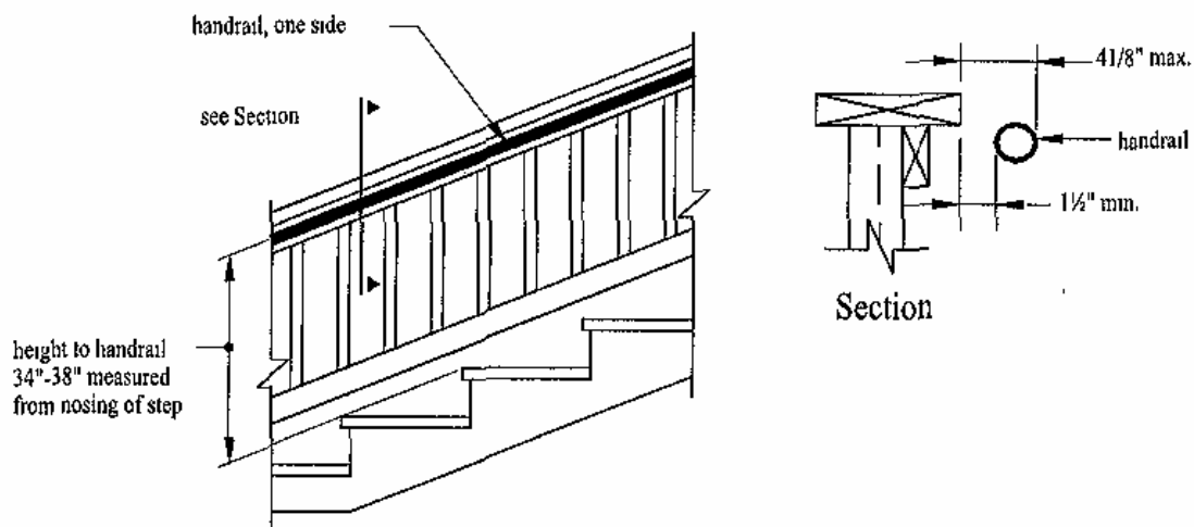
Figure 29: Stair handrail detail
