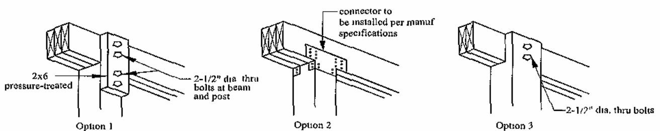
Figure 21: 6x6 inches post-to-beam connection
